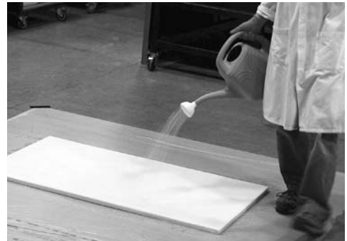
FIGURE 6: A WATERING CAN WITH A SHOWERHEAD SPOUT WILL CONTROL THE FLOW OF COLLOIDAL SILICA.
